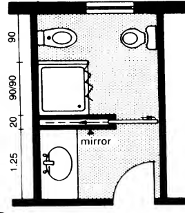
⑬ Separate washing area
